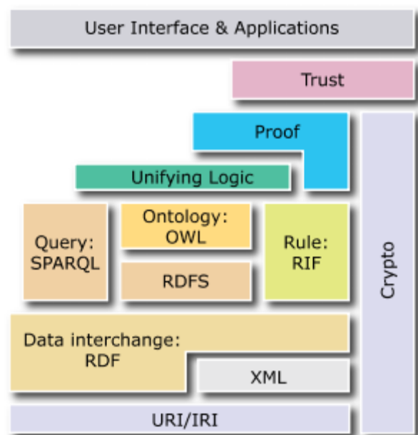
Figure 1. Semantic Web Layer Cake
